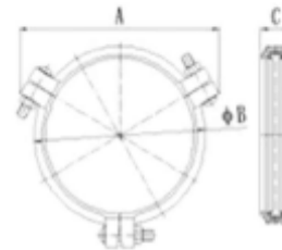
14" (355.6mm)-18" (480mm)
