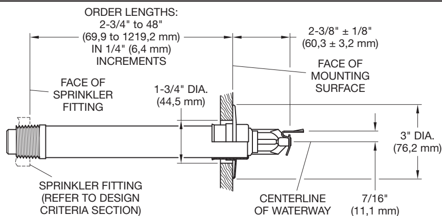
FIGURE 17 EXTENDED COVERAGE HORIZONTAL SIDEWALL SPRINKLER WITH STANDARD ESCUTCHEON TY3339 (3 MM BULB)
