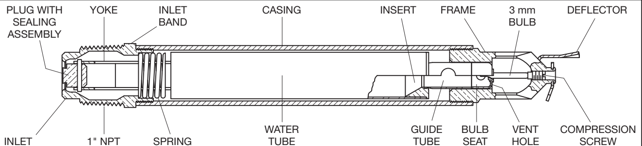
FIGURE 3 SERIES DS-1 STAINLESS STEEL DRY-TYPE EXTENDED COVERAGE HORIZONTAL SIDEWALL SPRINKLER TY3339 (3 MM BULB)
